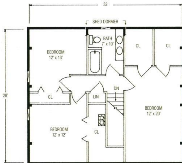
SECOND FLOOR 896 SQUARE FEET
