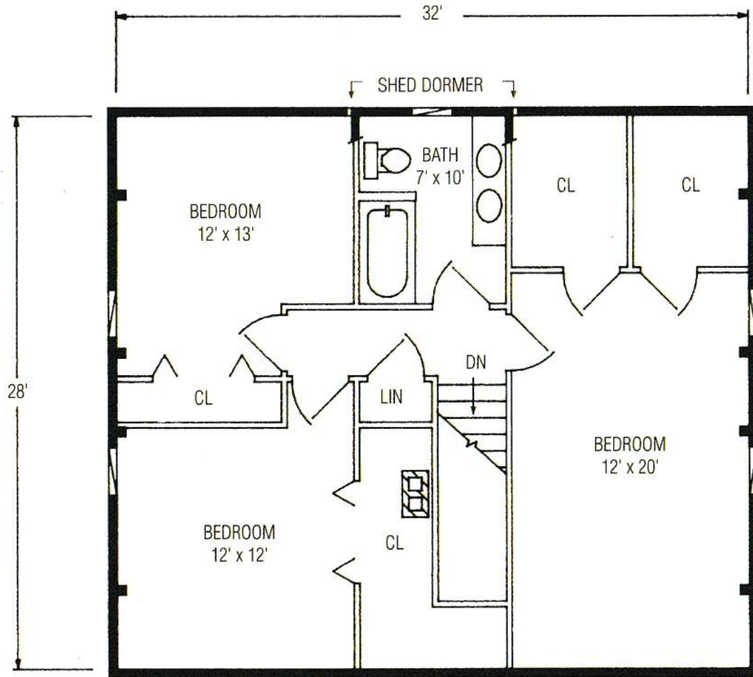
SECOND FLOOR 896 SQUARE FEET
